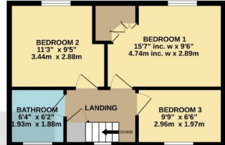
1ST FLOOR 390 sq.ft. (36.3 sq.m.) approx.
